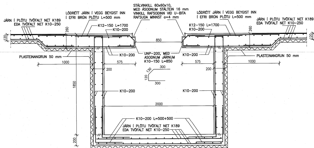
SNID 4-4 1:20
