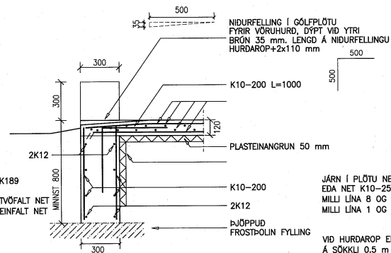
SNID 2-2 1:20
