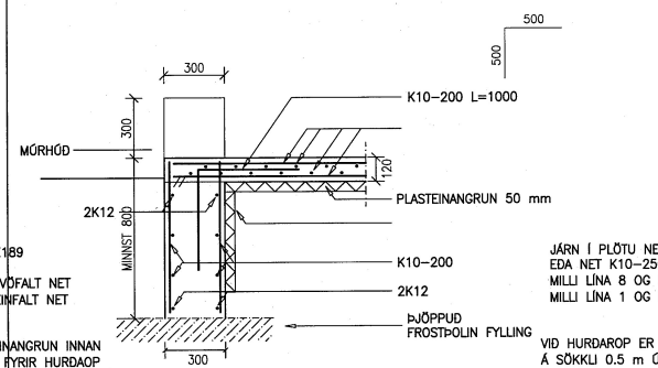
SNID 3-3 1:20
