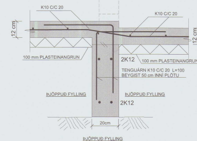
SNID F-F MKV. 1:10
