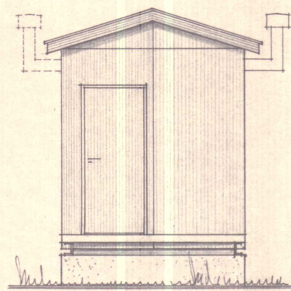
FRAMGAFL
