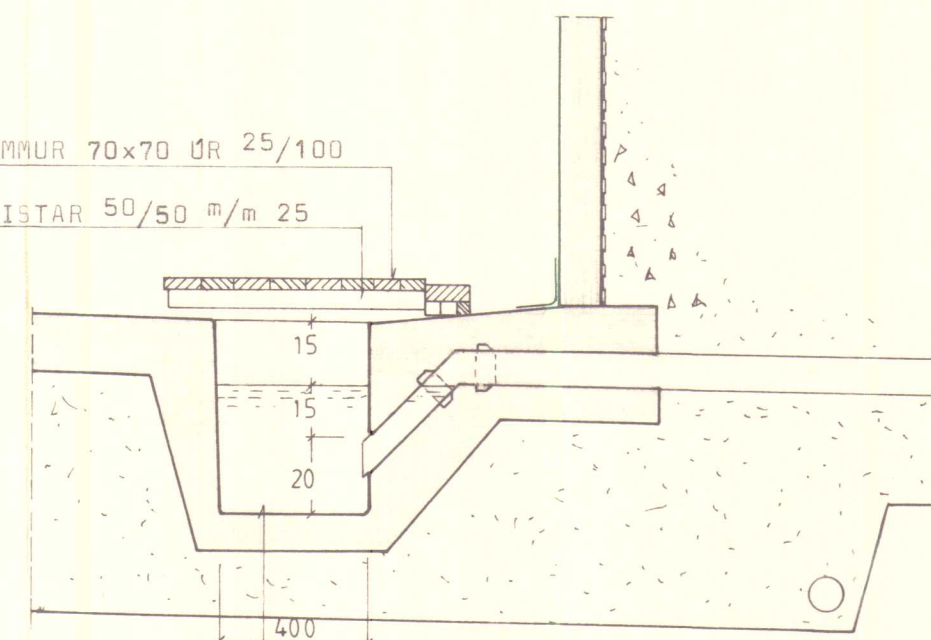
II M=1:20
