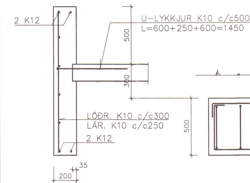
SNID C-C
