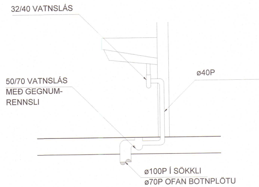
TENGING HANDLAUGA mkv 1:20
