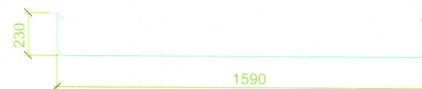
3. U Cradle Ø10 Amount: 40 Pieces./Foundation
