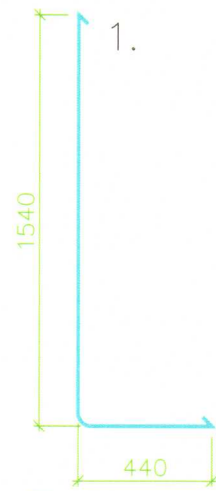
2. L Cradle Ø16 Amount: 12 Pieces./Foundation
