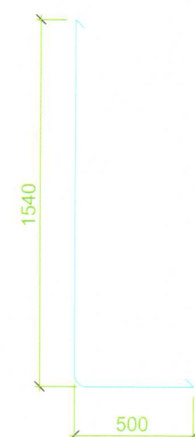
2. L Cradle Ø16 Amount: 16 Pieces./Foundation
