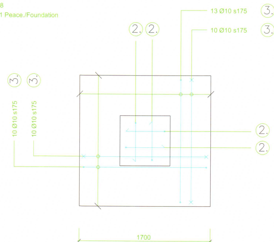
SECTION B-B (Reinforcement)
