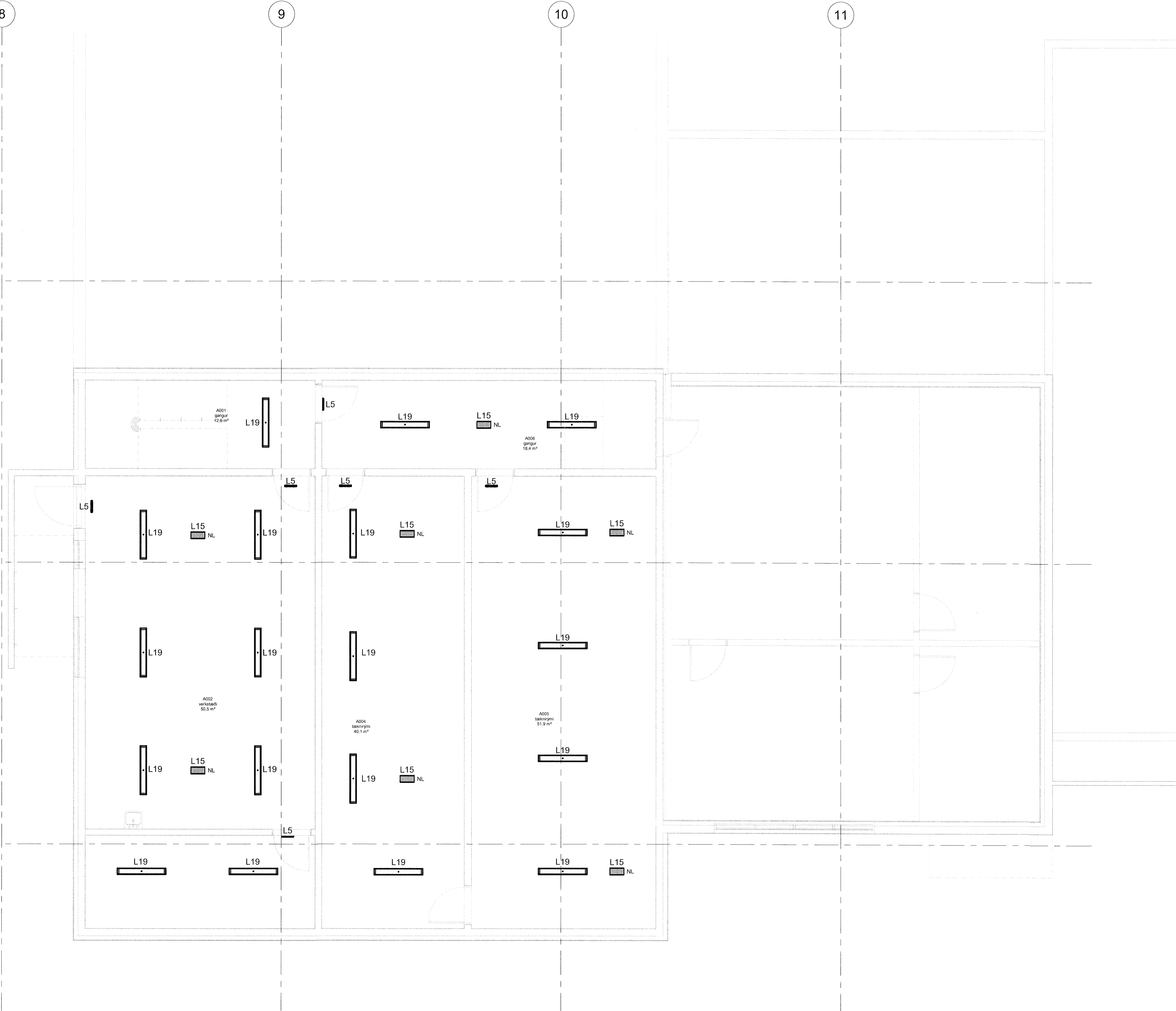
Lampaplan kjallari
