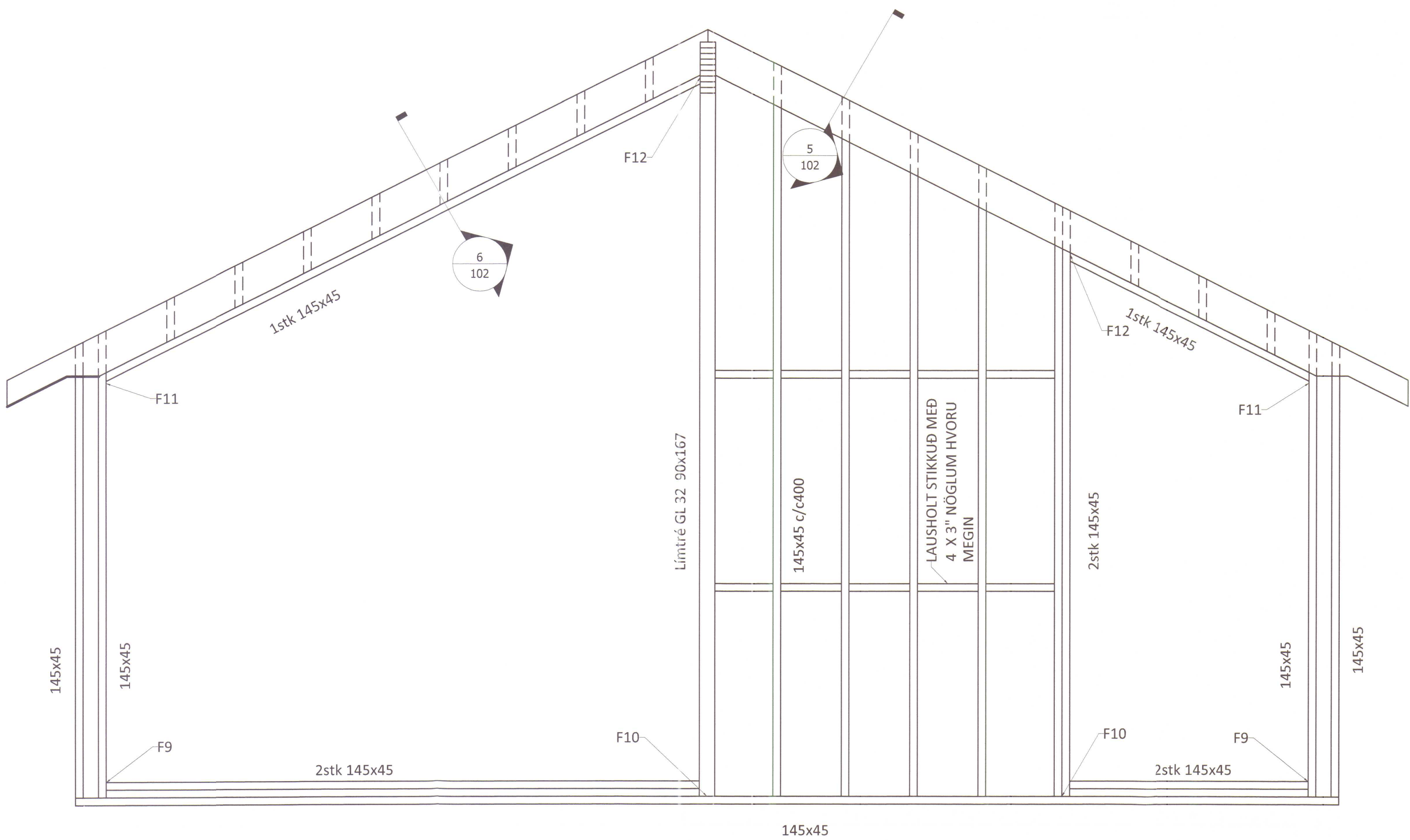
GAFL M 1:20
