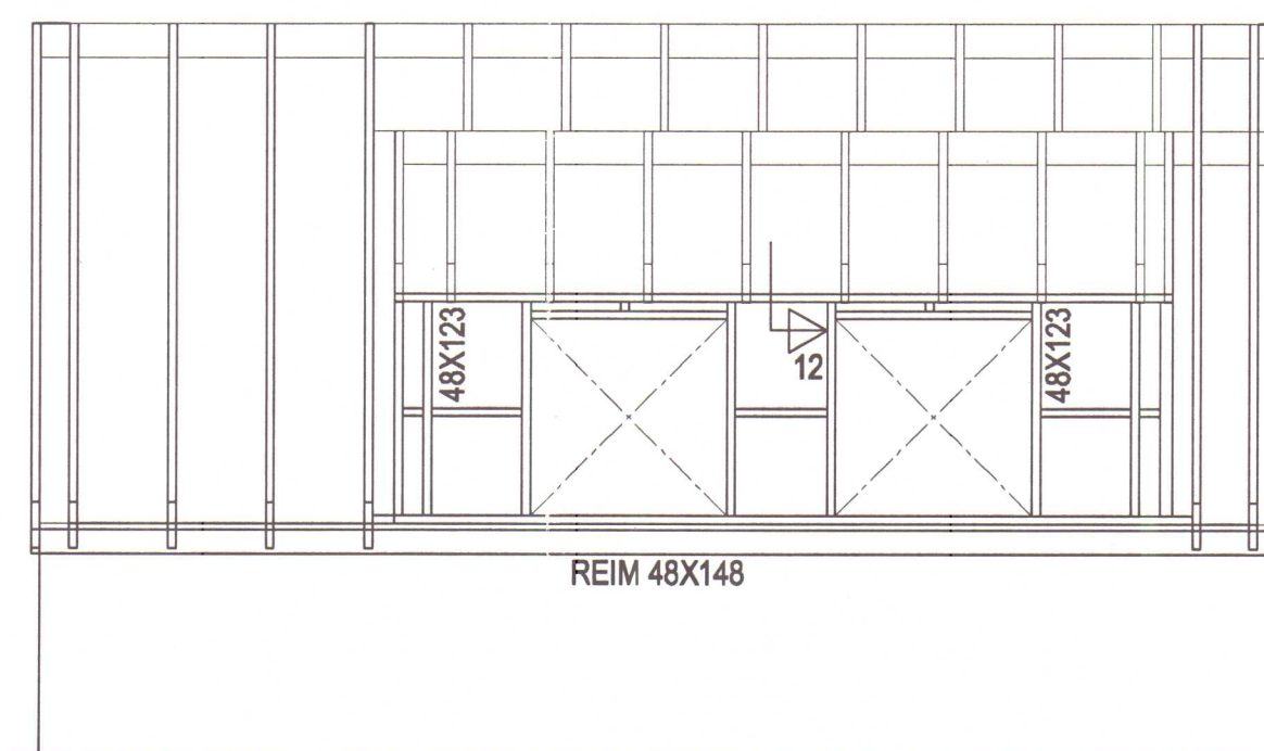
SNID 7-7 MKV. 1:50
