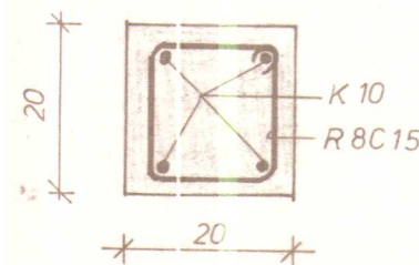
SNID C-C 1:10
