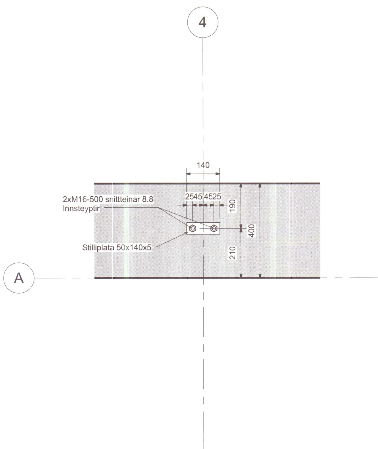
5 Festing, lagnvegg 1 : 10
