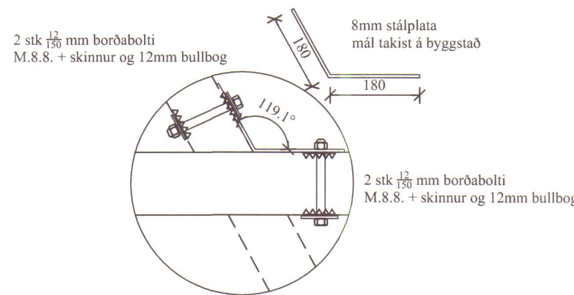
FESTING D . MK. 1:10
