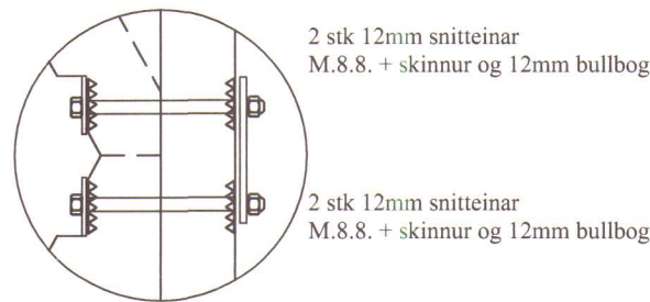
FESTING E . MK. 1:10
