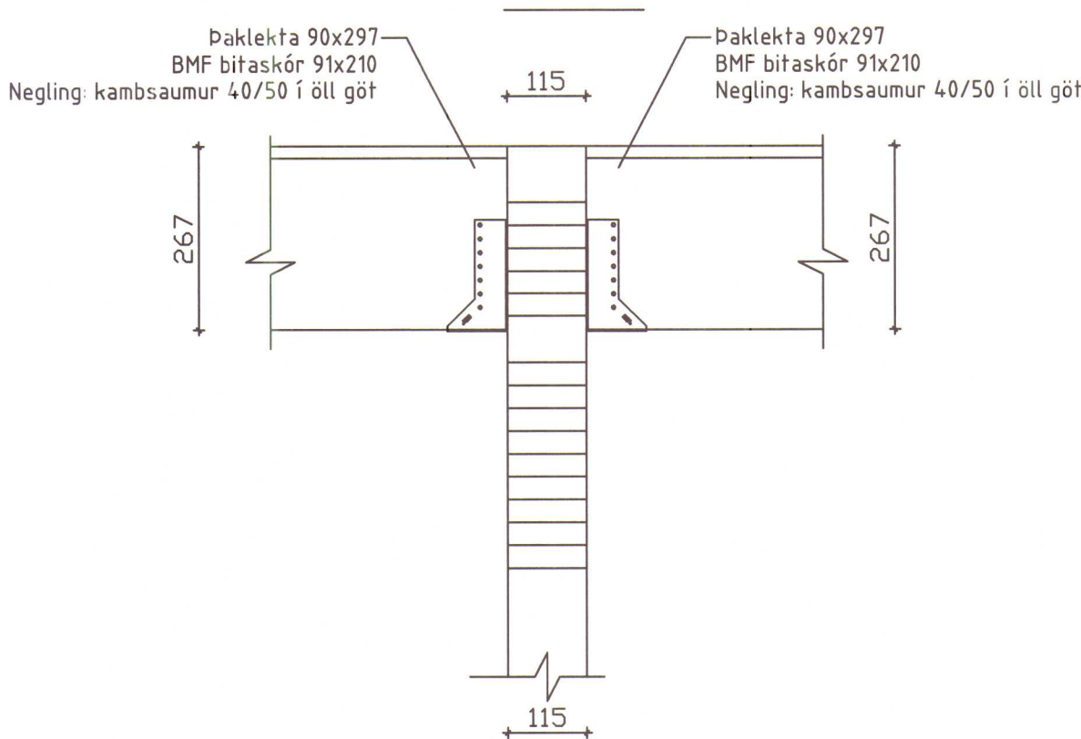
FESTING B MK. 1:10
