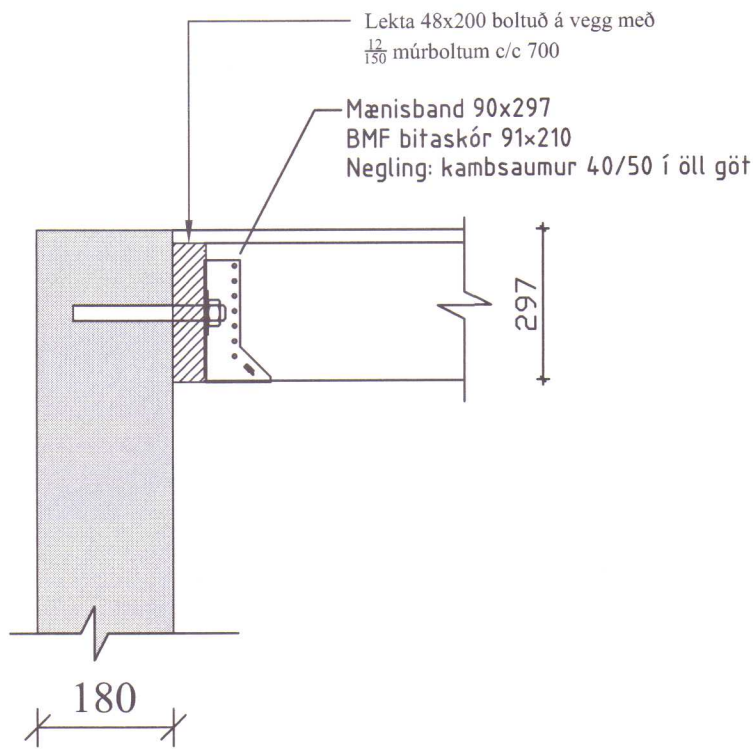
FESTING C MK. 1:10
