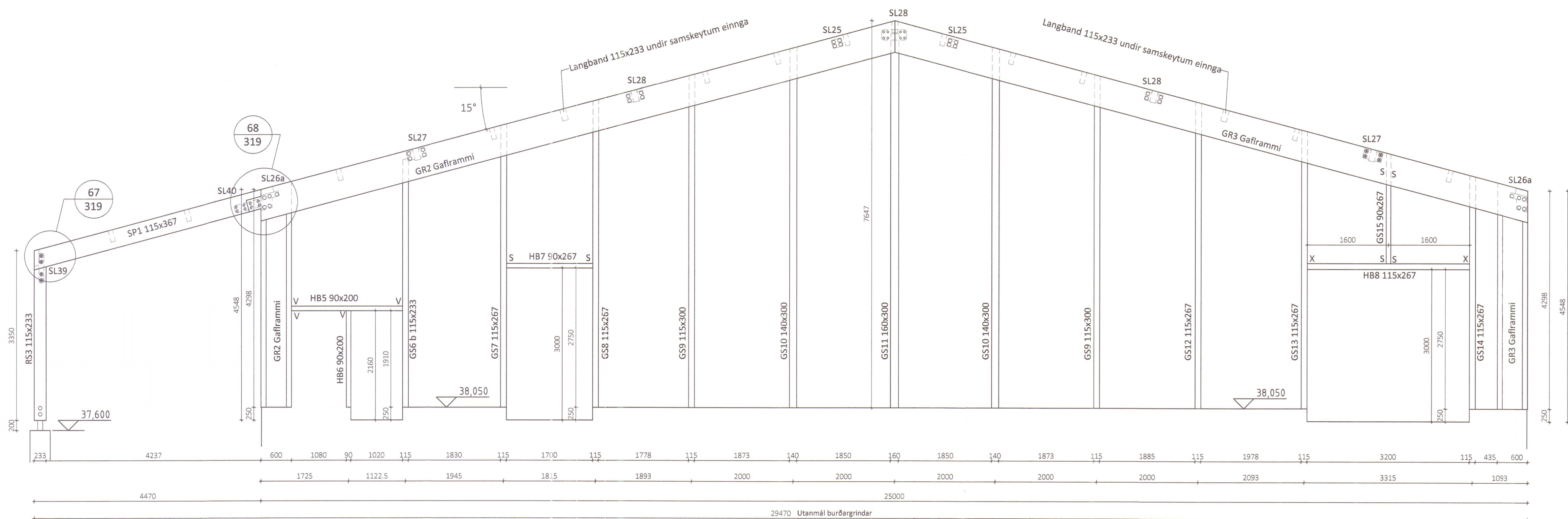
Gafl Reiðhöll - suður Mkv 1:50
