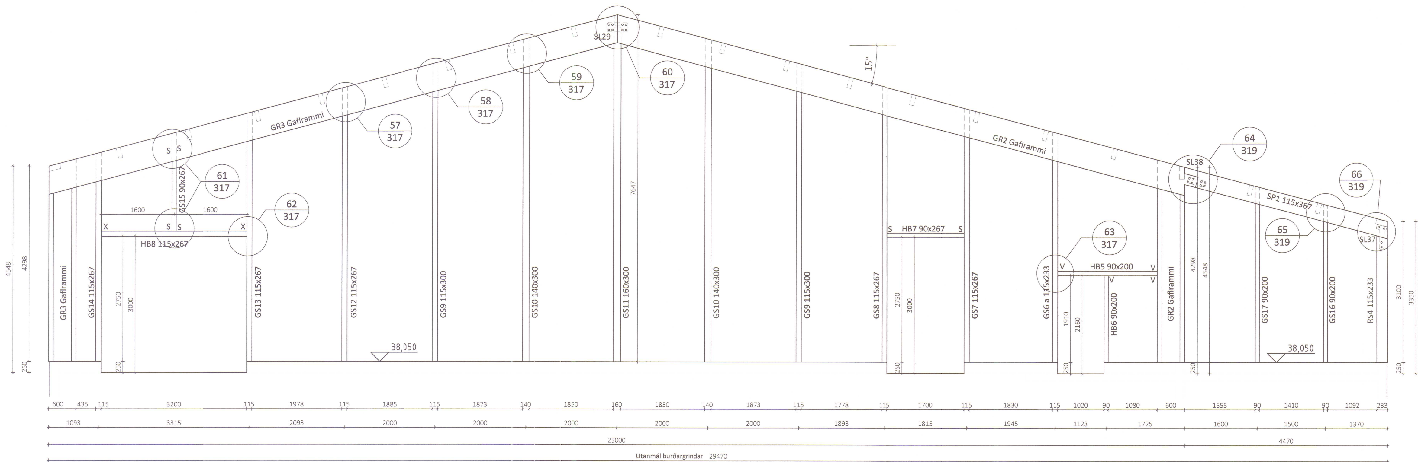
Gafl Reiðhöll - norður Mkv 1:50
